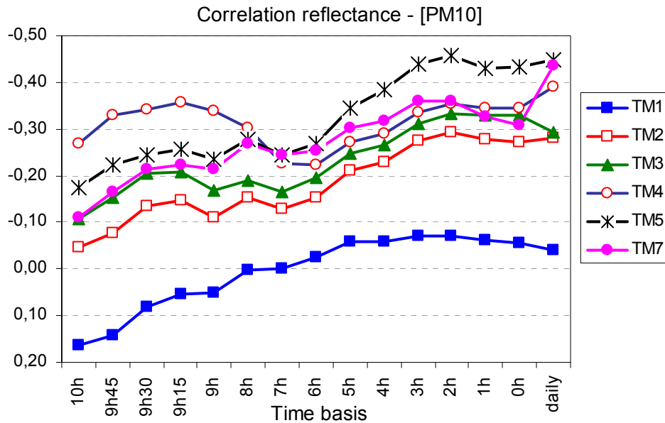
Figure 3: Linear correlation between integrated concentration of suspended particulates PM_{10} and reflectance derived from Landsat satellite- the x-axis and y-axis refer to the time basis and the correlation coefficients.
